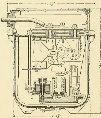
Fig. 67. Cross-Section of Westinghouse Unit Switch
